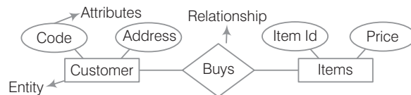
E-R Diagram
